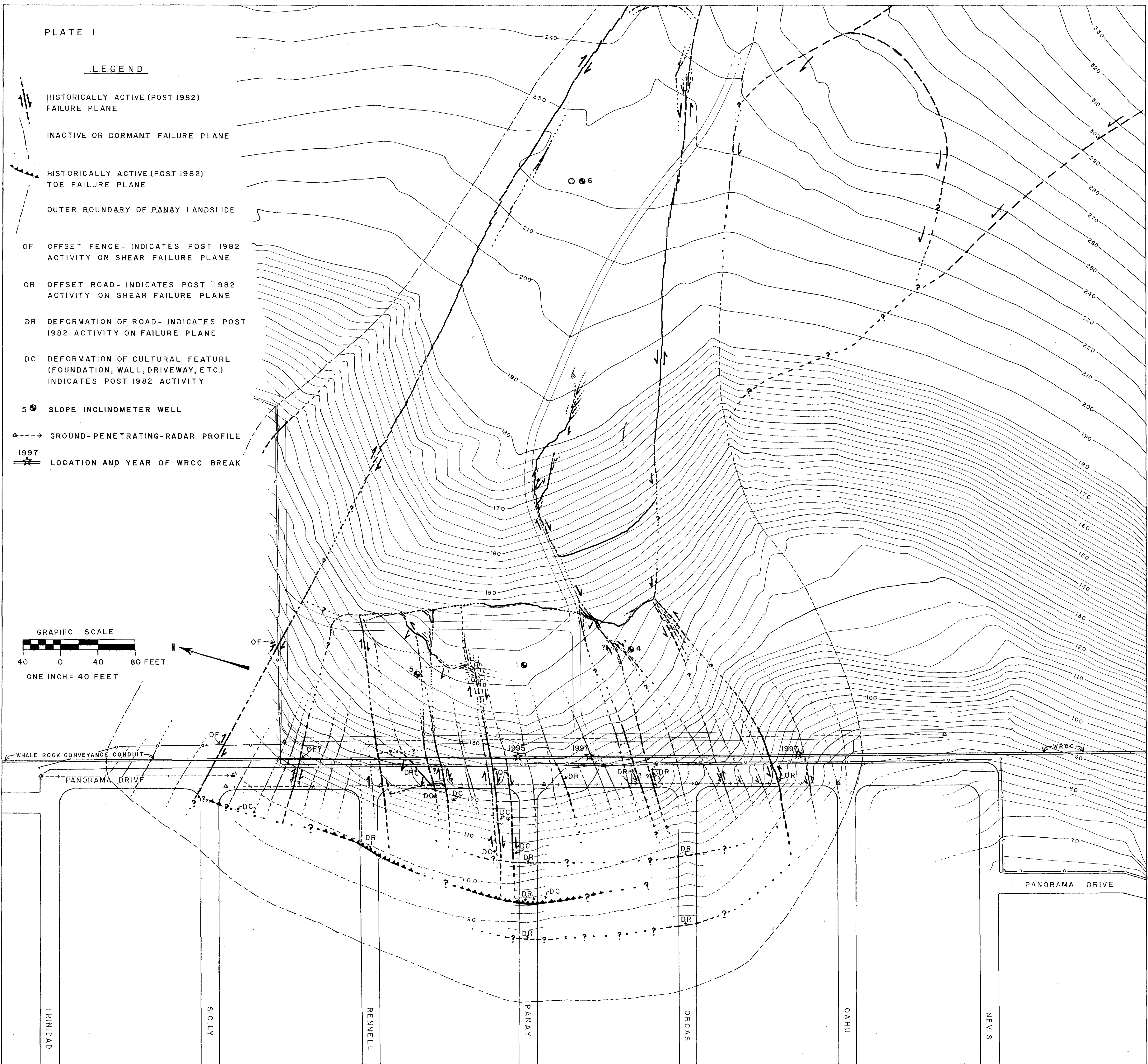
PARTIAL MAP OF HISTORICALLY ACTIVE AND DORMANT DEFORMATIONAL STRUCTURES IN THE PANAY LANDSLIDE ZONE, MORRO BAY, SAN LUIS OBISPO COUNTY, CALIFORNIA
